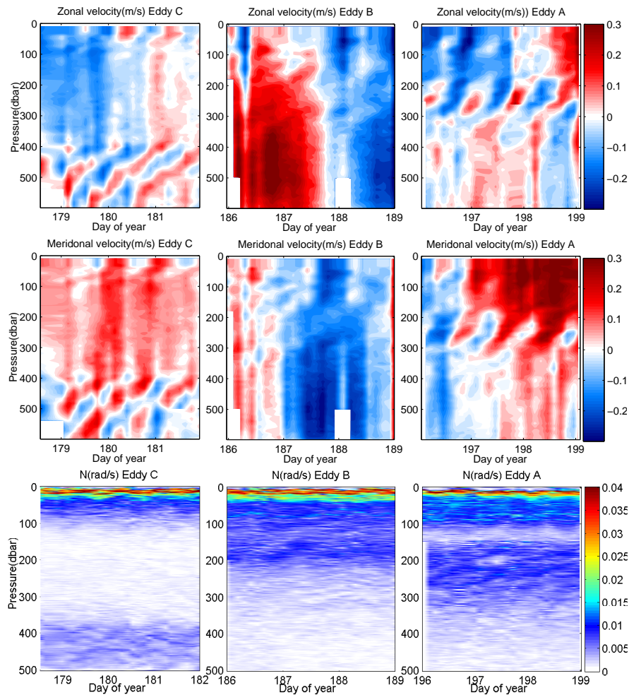
Fig. 3. Time depth plots of: (a) zonal velocity, (b) meridional velocity, (c) stratification profiles N(z) .
