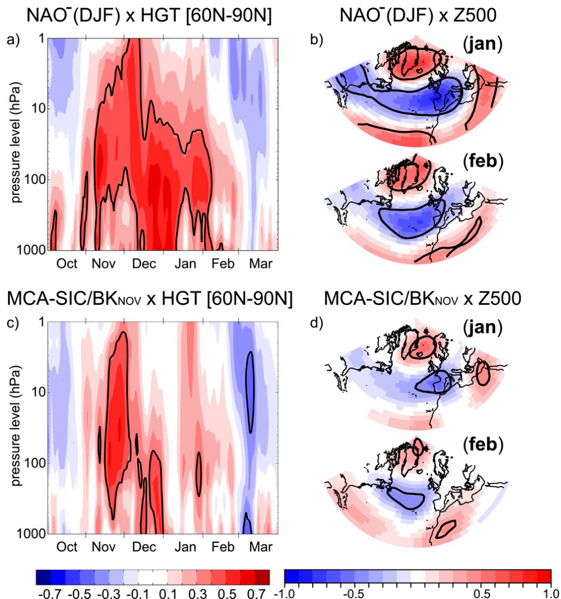
FIG. 10. (left) Correlation sections of detrended geopotential height anomalies averaged over the polar cap ( 60^{\circ} – 90^{\circ} N) with (a) the winter \text{NAO}^{-} index and (c) the \text{MCA-SIC/BK}_{\text{NOV}} expansion coefficient; the time axis is in daily values from 1 Oct to 31 Mar. (right) Correlation maps of detrended geopotential height anomalies at 500 hPa ( Z_{500} ) in January and February with (b) the winter \text{NAO}^{-} index and (d) the \text{MCA-SIC/BK}_{\text{NOV}} expansion coefficient. Statistically significant areas at 95% confidence level based on a two-tailed Student's t test are contoured.
