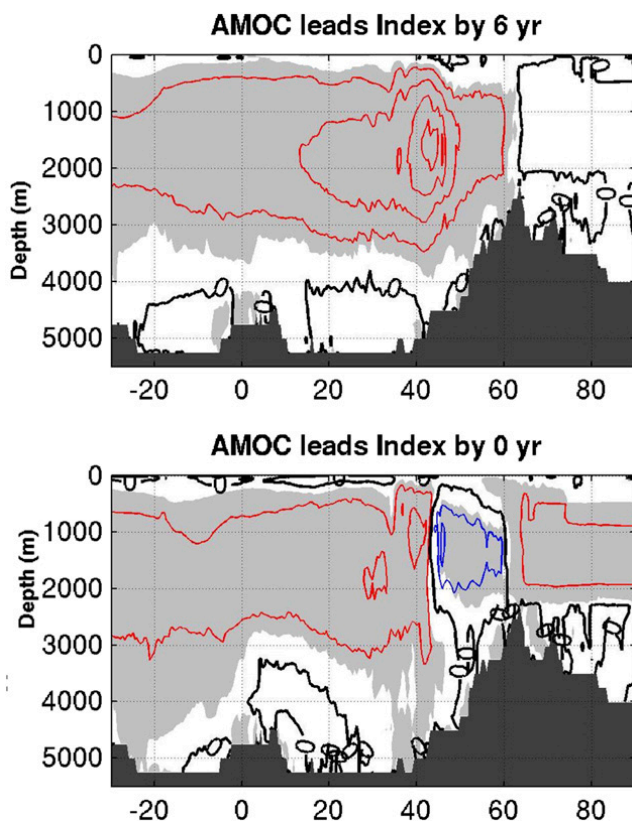
FIG. 14. Regression of the yearly AMOC [contour interval: 0.1 \text{ Sv} ; positive (red); negative (blue)] onto the -1 \times \text{GS-NAC} index (averaged latitude in 42^{\circ} – 47^{\circ}\text{W} ) when the AMOC (top) leads by 6 yr or (bottom) varies in phase. Note that the regressions correspond to a southward shift of the GS. Shading indicates 5% significance.
