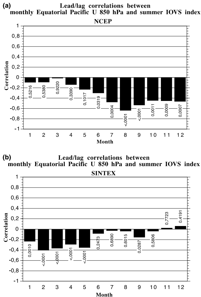
Fig. 14 Same as in Figs. 9a, b, but for the summer (June–September) IOVS index and the EQPAC monthly 850 hPa zonal wind time series from the NCEP reanalysis (1948–1998 period) and the SINTEX simulation (200 years)
