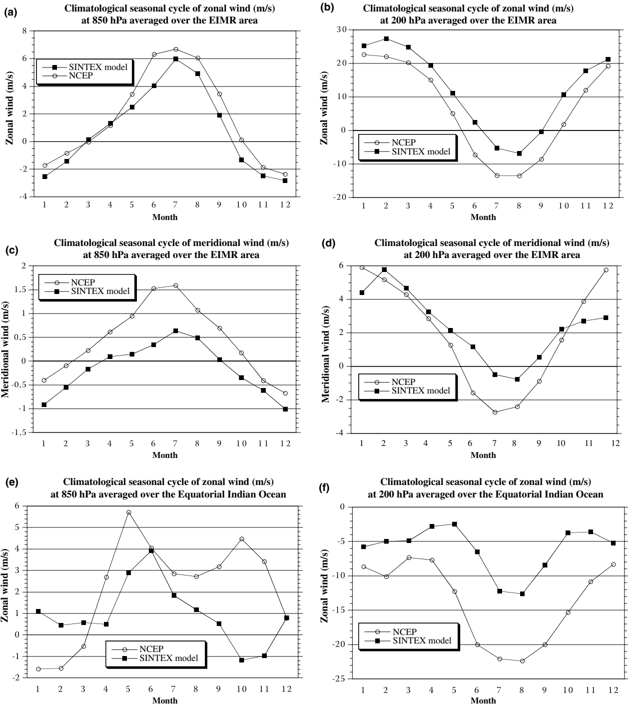
Fig. 5 Climatological seasonal cycle of 850 and 200 hPa wind components area-averaged over the EIMR (70°–110°E, 5°–30°N) and EQIO (60°–90°E, 2°S–2°N) areas for the NCEP reanalysis and the SINTEX model. a Zonal wind (850 hPa) over the EIMR
