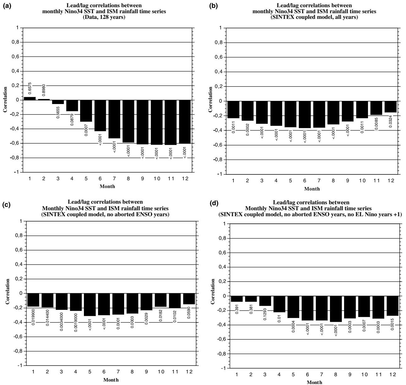
Fig. 9 Lead-lag correlations between IMR time series and the monthly Niño34 SST anomaly. a For the observations (1871–1998 period). b For the SINTEX simulation (200 years). c For the SINTEX simulation, but without aborted ENSO years. d For the SINTEX simulation, but without aborted ENSO years and years
