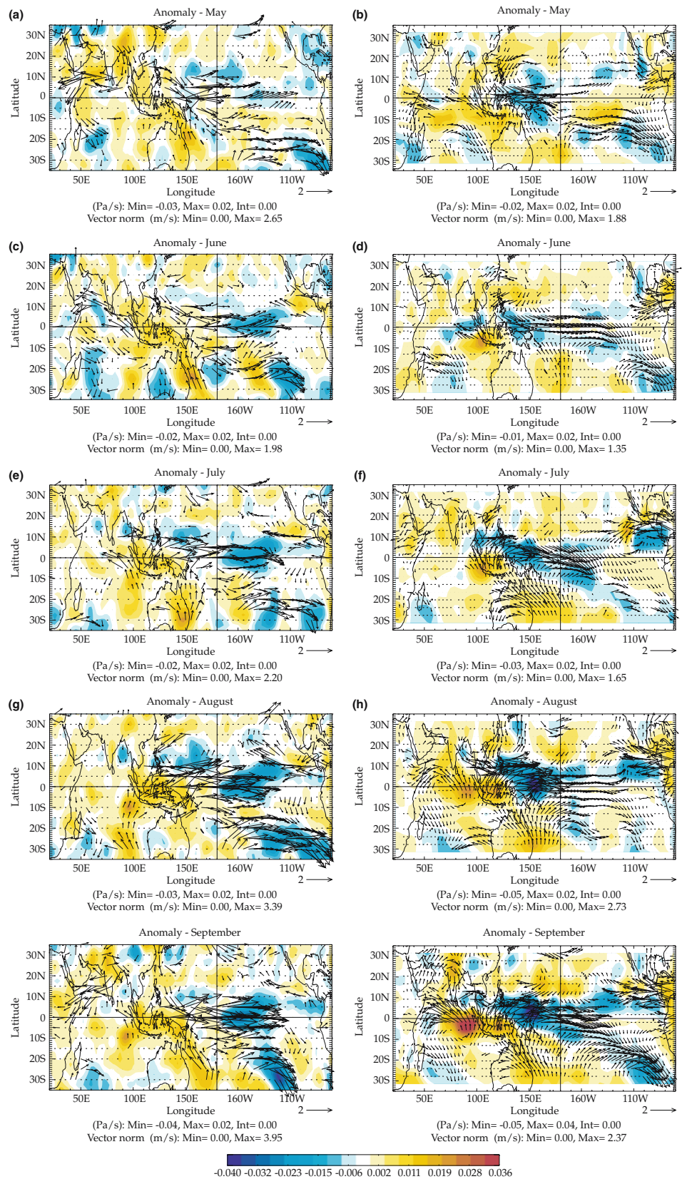
Fig. 8 Composite analysis of 850 hPa wind (m/s) and 500 hPa vertical pressure velocity (Pa/s) fields with respect to El Niño years from the NCEP reanalysis and the SINTEX simulation. The El Niño years are defined with the help of Niño34 SST anomaly (see text for more details). May, June, July, August and September composites during the El Niño years are presented. Only the 90% statistically significant 850 hPa wind anomalies are shown. a, c, e, g and i from the NCEP reanalysis. b, d, f, h and j from the SINTEX model
