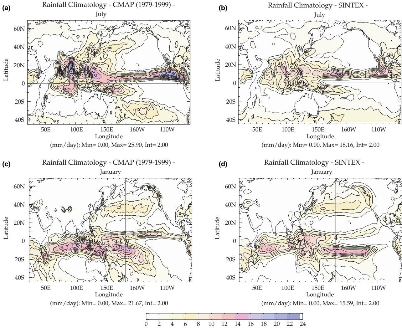
Fig. 3 Same as Fig. 1, but for the rainfall climatology
