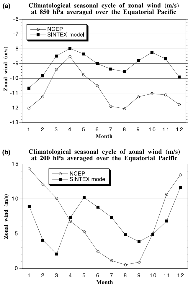
Fig. 7 Climatological seasonal cycle of 850 and 200 hPa zonal wind area-averaged over the EQPAC area ( 160^{\circ} – 130^{\circ} W, 2^{\circ} S– 2^{\circ} 5 N) for the NCEP reanalysis and the SINTEX model. a Zonal wind (850 hPa) over the EQPAC area. b Zonal wind (200 hPa) over the EQPAC area
