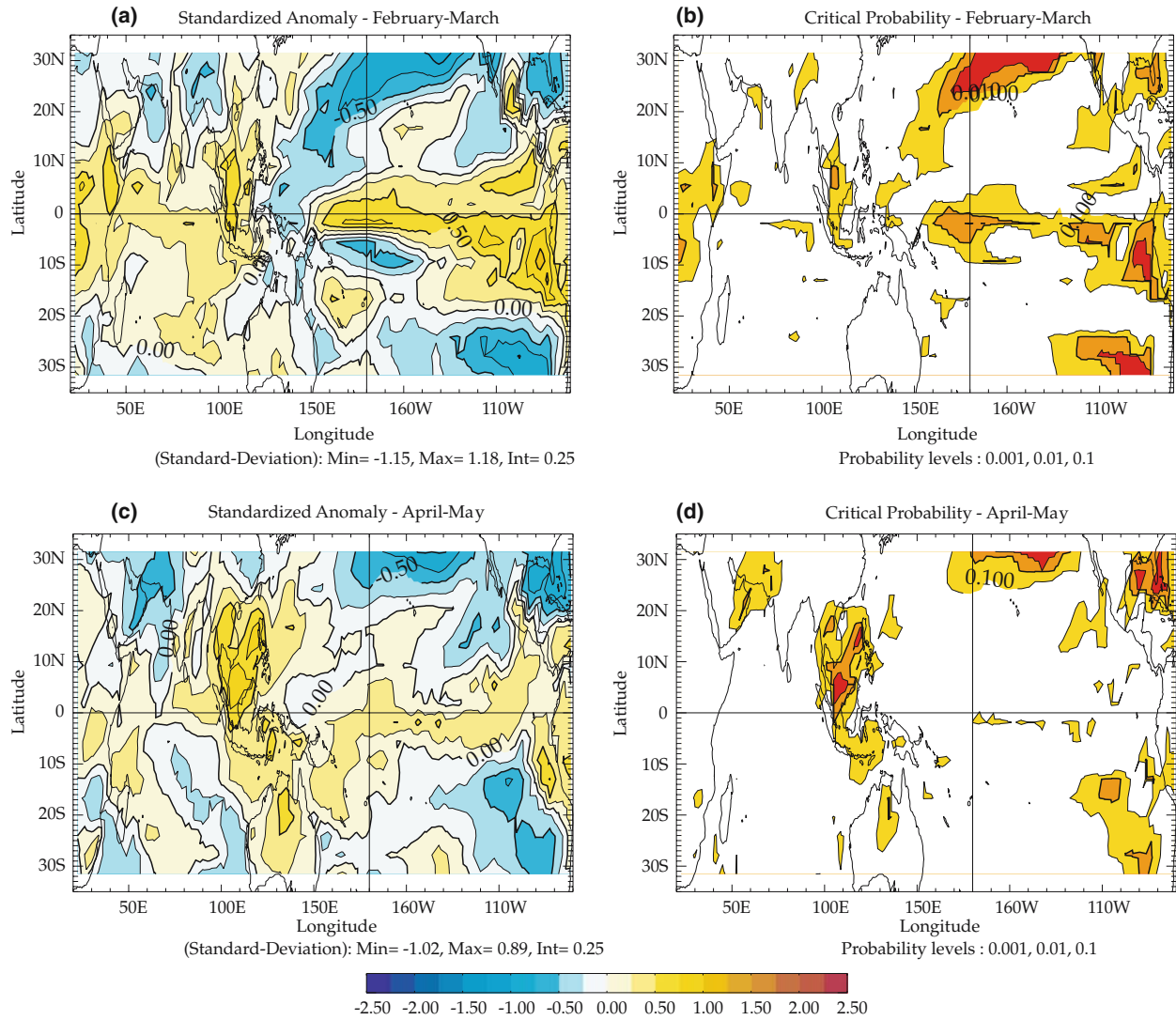
Fig. 13 a and c Composite analysis of February-March and April-May SST fields with respect to weak ISMs which are not regular or aborted El Niño years in the SINTEX simulation. b and d
