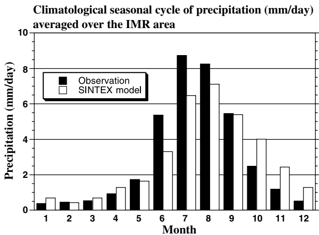
Fig. 4 Climatological seasonal cycle of precipitation (mm/day) averaged over the IMR area for the observations and the SINTEX model. The observed IMR is from Parthasarathy et al. (1995). In the simulation, IMR is defined as the area-averaged precipitation over all land grid-points in the domain 75°E–85°E, 10°N–25°N
