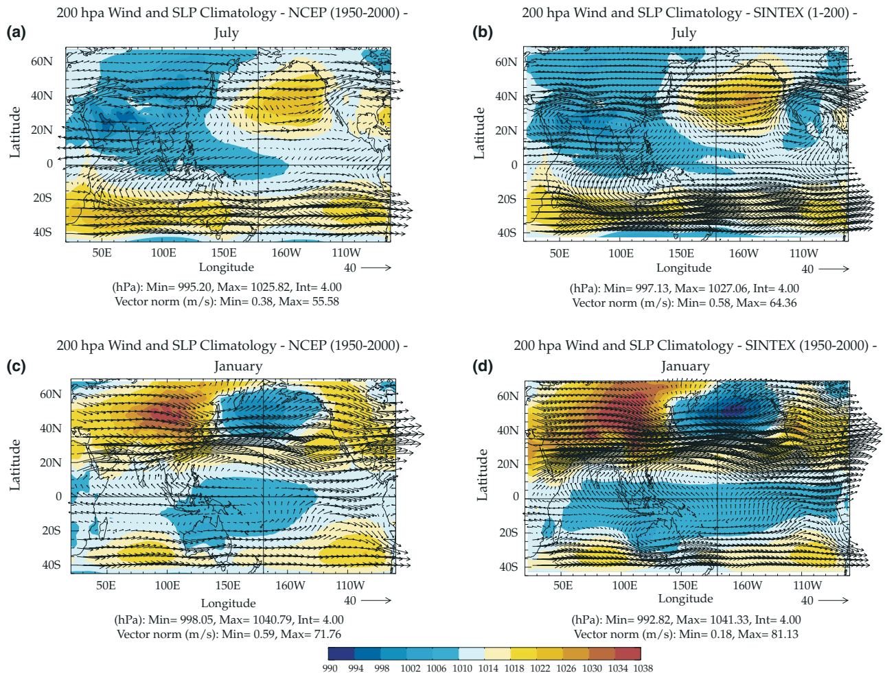
Fig. 2 Same as Fig. 1, but for the 200 hPa wind and SLP climatology
