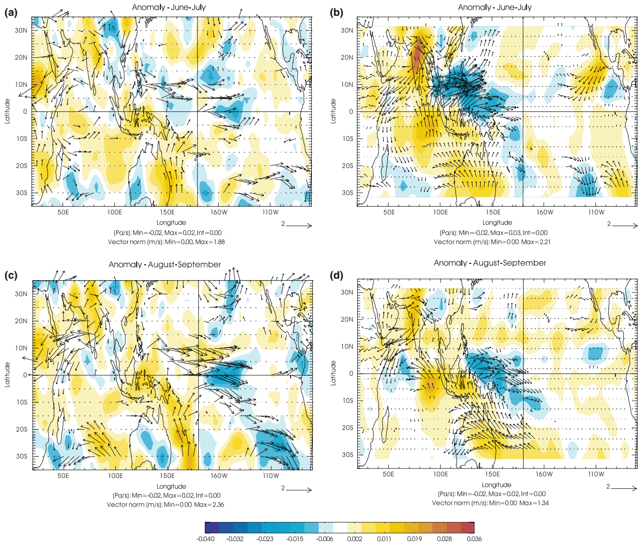
Fig. 10 Composite analysis of 850 hPa wind (m/s), and 500 hPa vertical pressure velocity (Pa/s) fields with respect to weak ISM years from the NCEP reanalysis (1948–1998 period) and the SINTEX simulation. The weak ISM years are defined with the help of the IMR index. The weak ISMs, which are also aborted El Niño years have been excluded from the composites in the simulation
