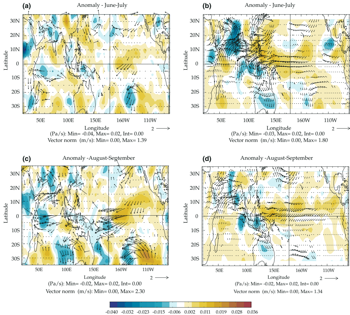
Fig. 11 Same as Fig. 10, but for the strong ISMs.
