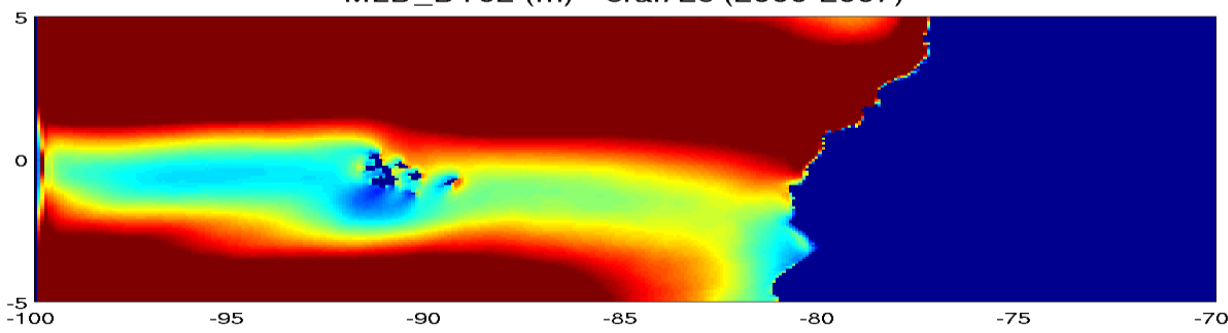
MLD_DT02 (m) - erai72c (2000-2007)
