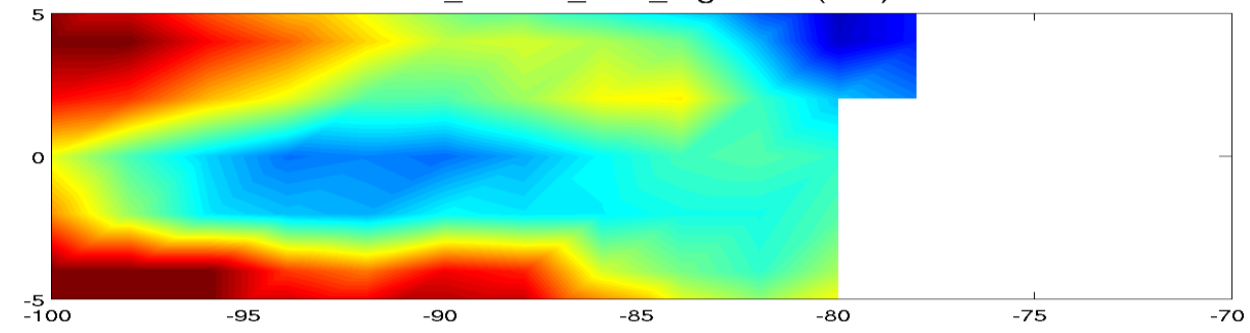
mld_DR003_c1m_reg2.0.nc (mld)
