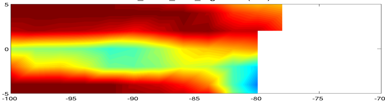
mld_DT02_c1m_reg2.0.nc (mld)
