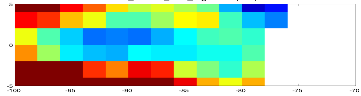
mld_DR003_c1m_reg2.0.nc (mld)
