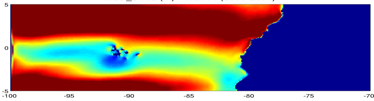
MLD_DT02 (m) - erai70c (2000-2007)
