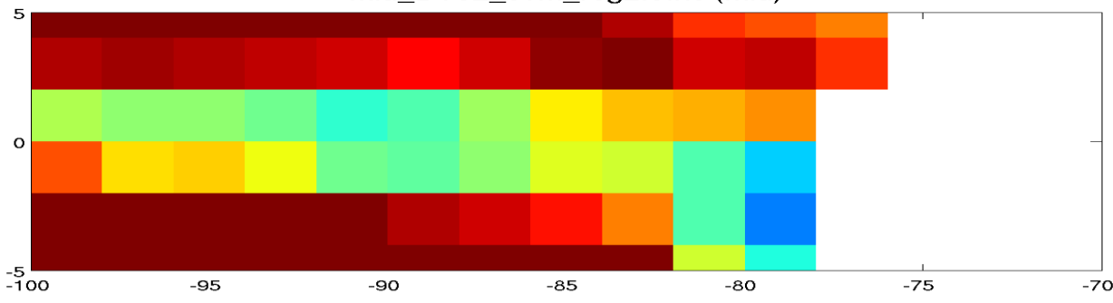
mld_DT02_c1m_reg2.0.nc (mld)
