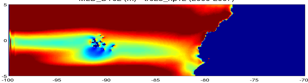
MLD_DT02 (m) - tr025_np12 (2000-2007)
