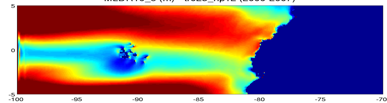
MLDR10_3 (m) - tr025_np12 (2000-2007)
