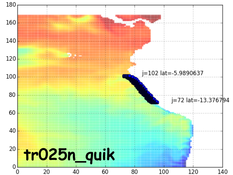
tr025n_quikubs / 3240 particules: position initiale le 31 12 2008
