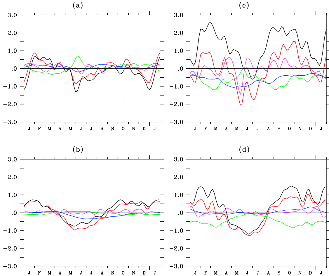
Figure 9. Time plots of 1997–2000 mean seasonal cycles, in ^{\circ}\text{C month}^{-1} . Plots (left) at 23^{\circ}\text{W} : (a) 4^{\circ}\text{N} – 8^{\circ}\text{N} average and (b) 4^{\circ}\text{S} – 8^{\circ}\text{S} average and (right) at 3^{\circ}\text{E} : (c) 4^{\circ}\text{N} – 8^{\circ}\text{N} average and (d) 4^{\circ}\text{S} – 8^{\circ}\text{S} average. The red line is heat storage, the black line is atmospheric forcing, the green line is subsurface, the purple line is horizontal advection by eddies, and the blue line is zonal and meridional advections by low-frequency currents.
