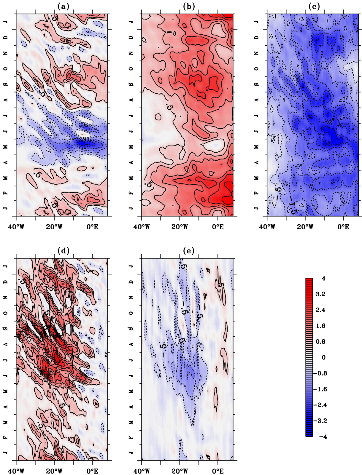
Figure 8. Longitude-time plots along the equator (2°N–2°S average) of 1997–2000 mean seasonal cycles of (a) heat storage, (b) atmospheric forcing, (c) tendencies due to vertical exchanges with the subsurface ocean (sum of vertical advection, vertical diffusion at the base of the mixed layer, and entrainment), (d) eddies (high-frequency horizontal advection plus lateral diffusion), and (e) zonal and meridional advections by low-frequency currents (contours every 0.5°C month -1 between -2°C month -1 and 2°C month -1 and every 1°C month -1 after; the thick line is zero). All the trends are smoothed with a 25-day Hanning filter.
