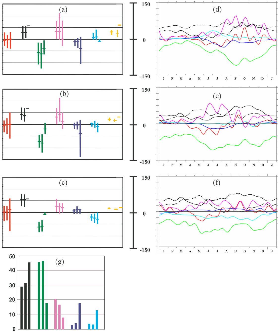
Figure 10. Heat budget annual tendencies ( \text{W m}^{-2} ) and mixed layer depth (m, in yellow) for CLIPPER (left bars), ORCA05 (middle bars) and PIRATA (right bars) at (a) 35^{\circ}\text{W}-0^{\circ}\text{N} , (b) 23^{\circ}\text{W}-0^{\circ}\text{N} , and (c) 10^{\circ}\text{W}-0^{\circ}\text{N} . The PIRATA heat budget values are from Foltz et al. [2003]. The bars represent minimum, maximum (vertical bars), and mean (horizontal bars). Seasonal cycle of CLIPPER tendencies around (d) 35^{\circ}\text{W}-0^{\circ}\text{N} , (e) 23^{\circ}\text{W}-0^{\circ}\text{N} , and (f) 10^{\circ}\text{W}-0^{\circ}\text{N} , in \text{W m}^{-2} . (g) Relative contributions (%) of the various terms for the total budget in CLIPPER (left bars), ORCA05 (middle bars), and PIRATA (right bars). Heat storage is given in red, forcing is given in black (dashed line is the damping contribution), subsurface is given in green, horizontal advection by eddies is given in purple, zonal advection by low-frequency currents is given in dark blue, and meridional advection by low-frequency currents is given in light blue.
