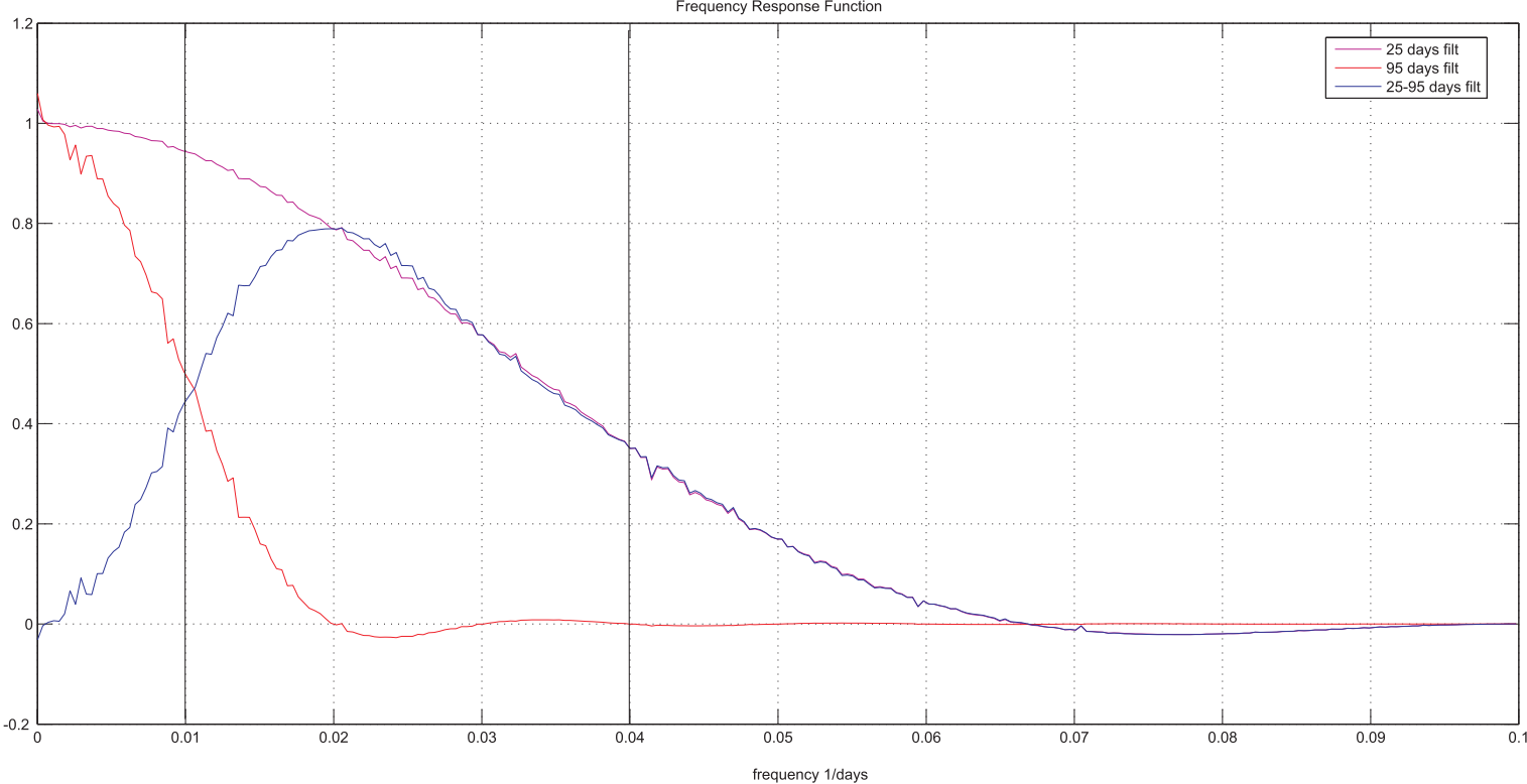
Figure 3: Response function of the filter performed as the ratio between the Fourier Transform of the filtered signal and the Fourier Transform of the original signal.
