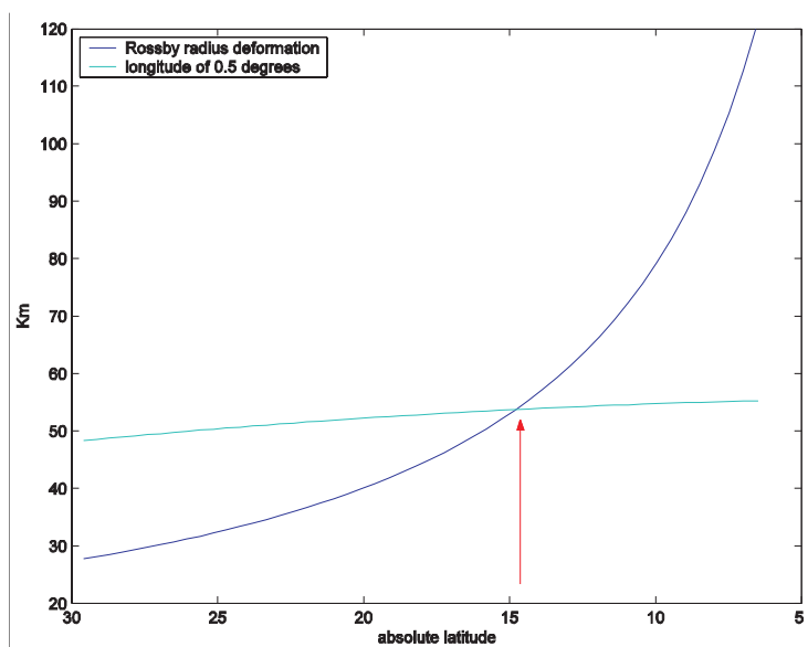
Figure 1: Rossby radius of deformation for a given phase speed c=2\text{m/s} and the distance of the 0.5^\circ longitude versus the latitude.
