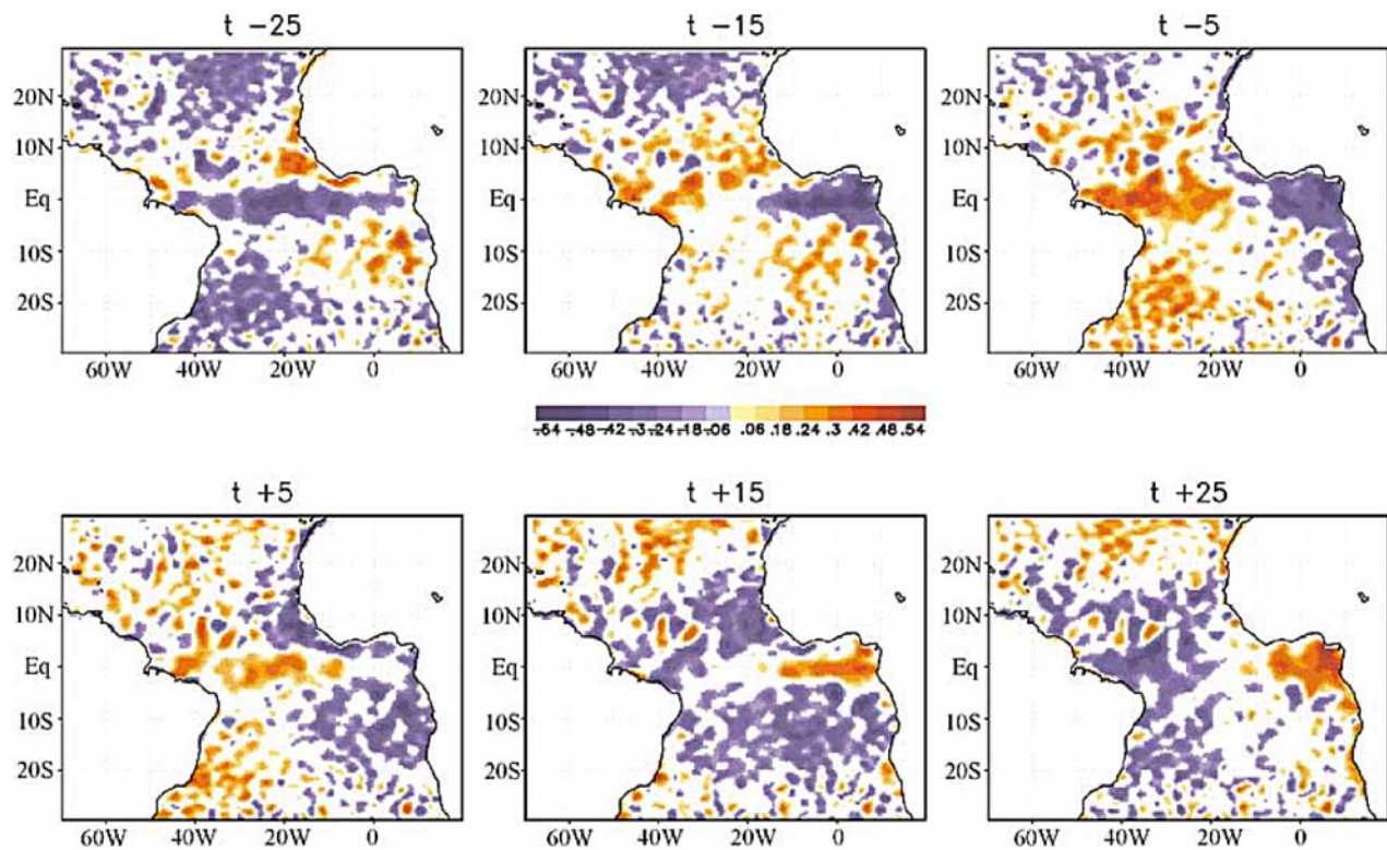
Figure 7. Regression of the observed intraseasonal SSH anomalies over the whole tropical Atlantic on the leading EEOF mode from Figure 6 at different lags (in cm). Only statistically significant areas at 95% confidence limit are plotted.
