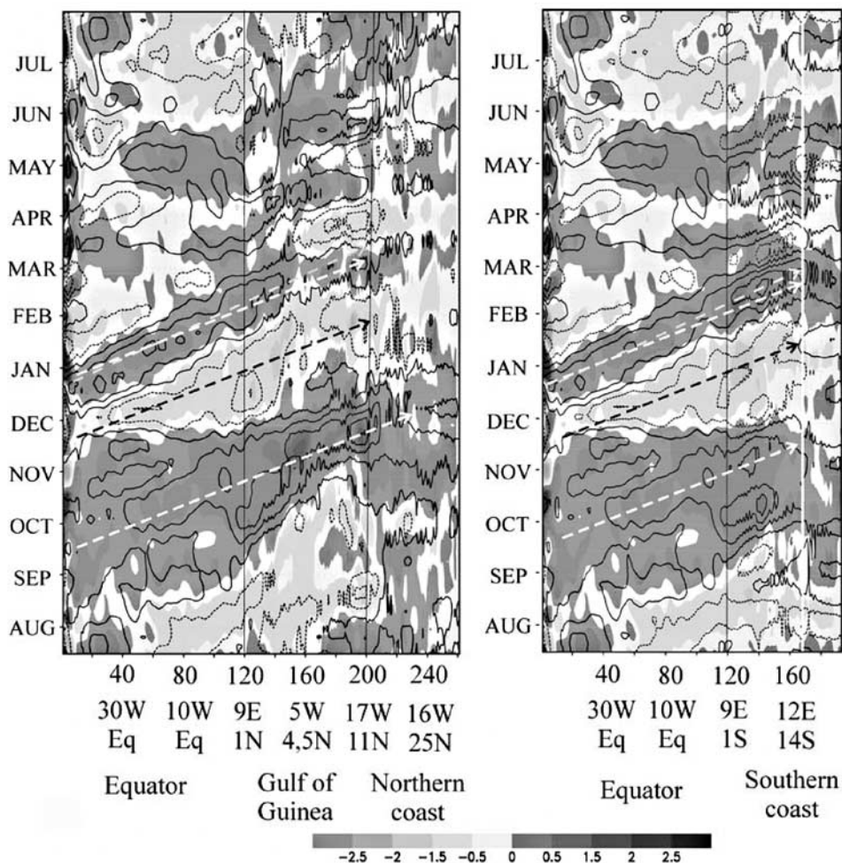
Figure 5a. Climatology of the intraseasonal SSH anomalies (in cm) for the observations (shaded areas) and the model (contour lines, contour interval (CI) is 0.5, the zero line has been removed) for (left) the north wave track and (right) the south wave track. The arrows correspond to 1.8 (white and black lines) and 1.6 m/s (gray line) propagation phase speeds.
