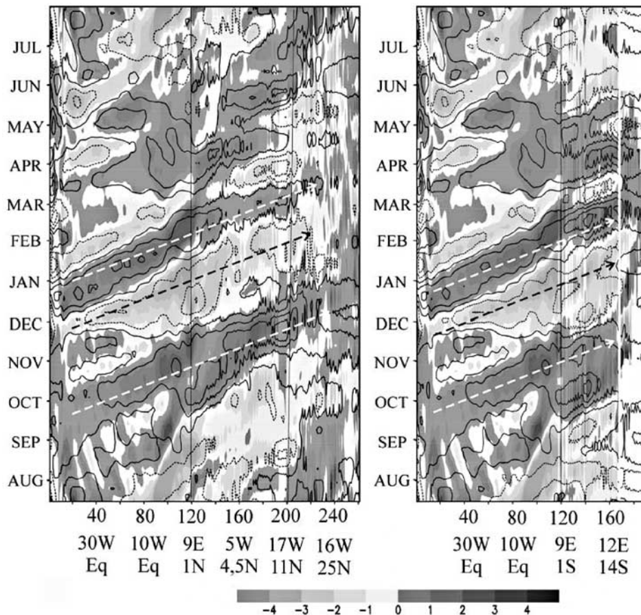
Figure 5c. Climatology of the intraseasonal 18^{\circ}\text{C} isotherm depth anomalies (shaded areas, in m) and modeled intraseasonal SSH anomalies (contour lines, CI is 0.5 cm, the zero line has been removed) for (left) the north wave track and (right) the south wave track. The arrows correspond to 1.8 m/s propagation phase speed.
