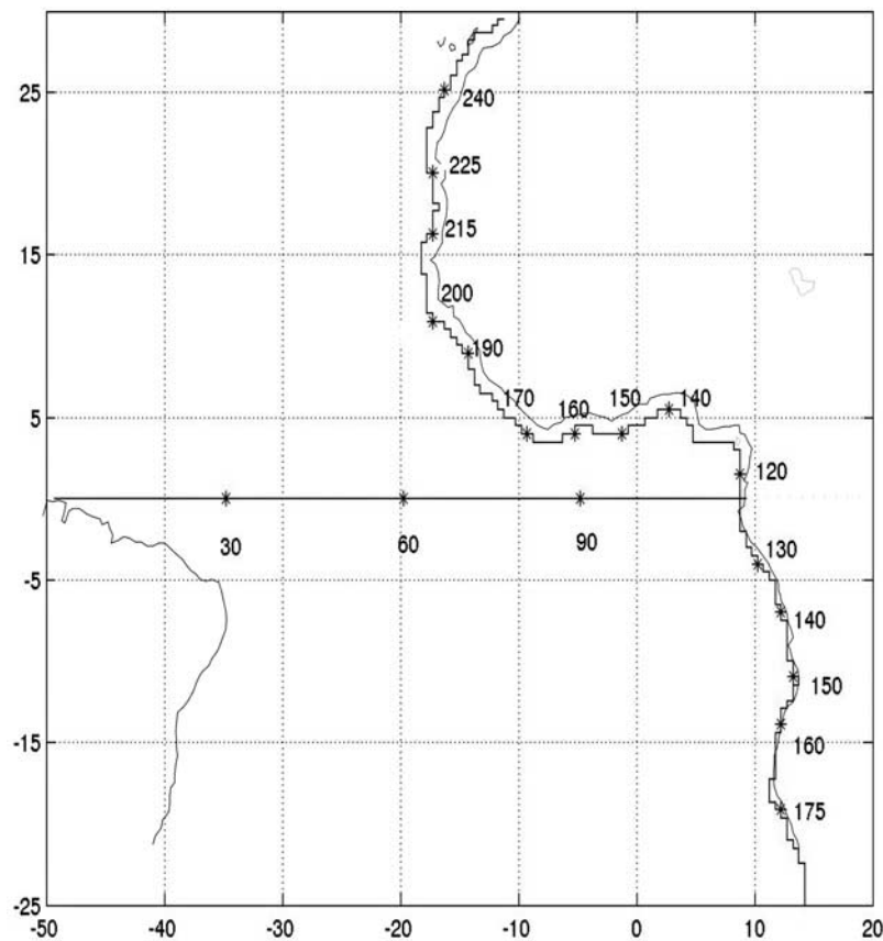
Figure 1b. Map of the grid points along the equator and the African coast used in the study of Kelvin wave tracks.
