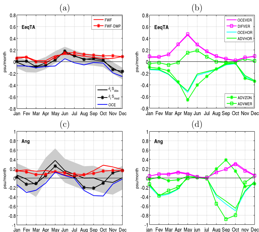
Figure 10. As Figure 4 at EeqTA (7°S:3°N/15°W:2°E) and Ang (7:17°S/8:14°E).
