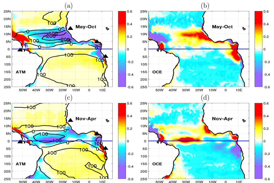
Figure 2. (a) Atmospheric and (b) oceanic contributions to the MLS budget. (c, d) The same as Figures 2a and 2b for November–April mean. Units are in psu/mois. Contours on Figures 2a and 2c are E-P in mm/mois. Triangles in Figures 2a and 2c are rivers positions (Gambia, Niger, Congo, and Amazon).
