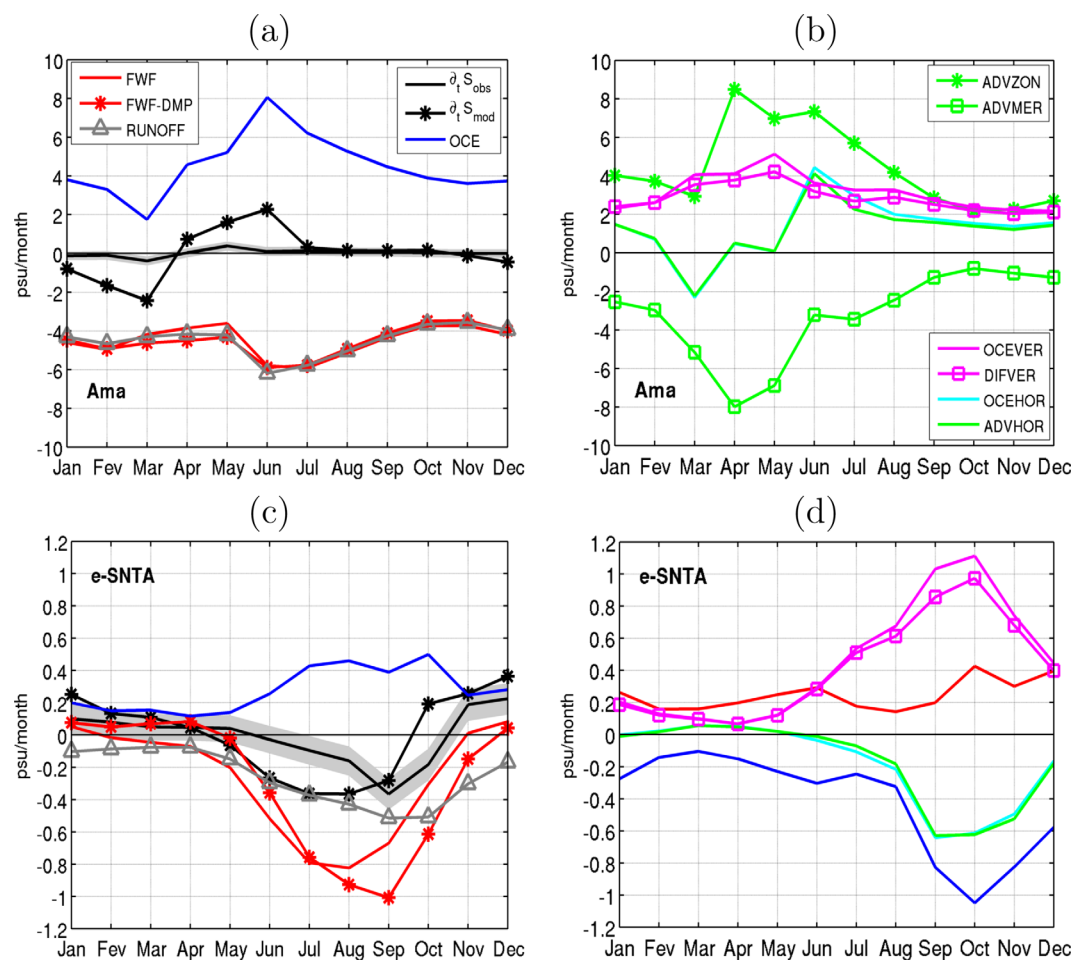
Figure 9. As Figure 4 except for (b) where horizontal advection is separated into zonal and meridional components: Ama ( 3^{\circ}\text{N} : 7^{\circ}\text{S} : 51:40^{\circ}\text{E} ) and e-SNTA ( 10:17^{\circ}\text{N} : 20:5^{\circ}\text{W} ). Units are in psu/month.
