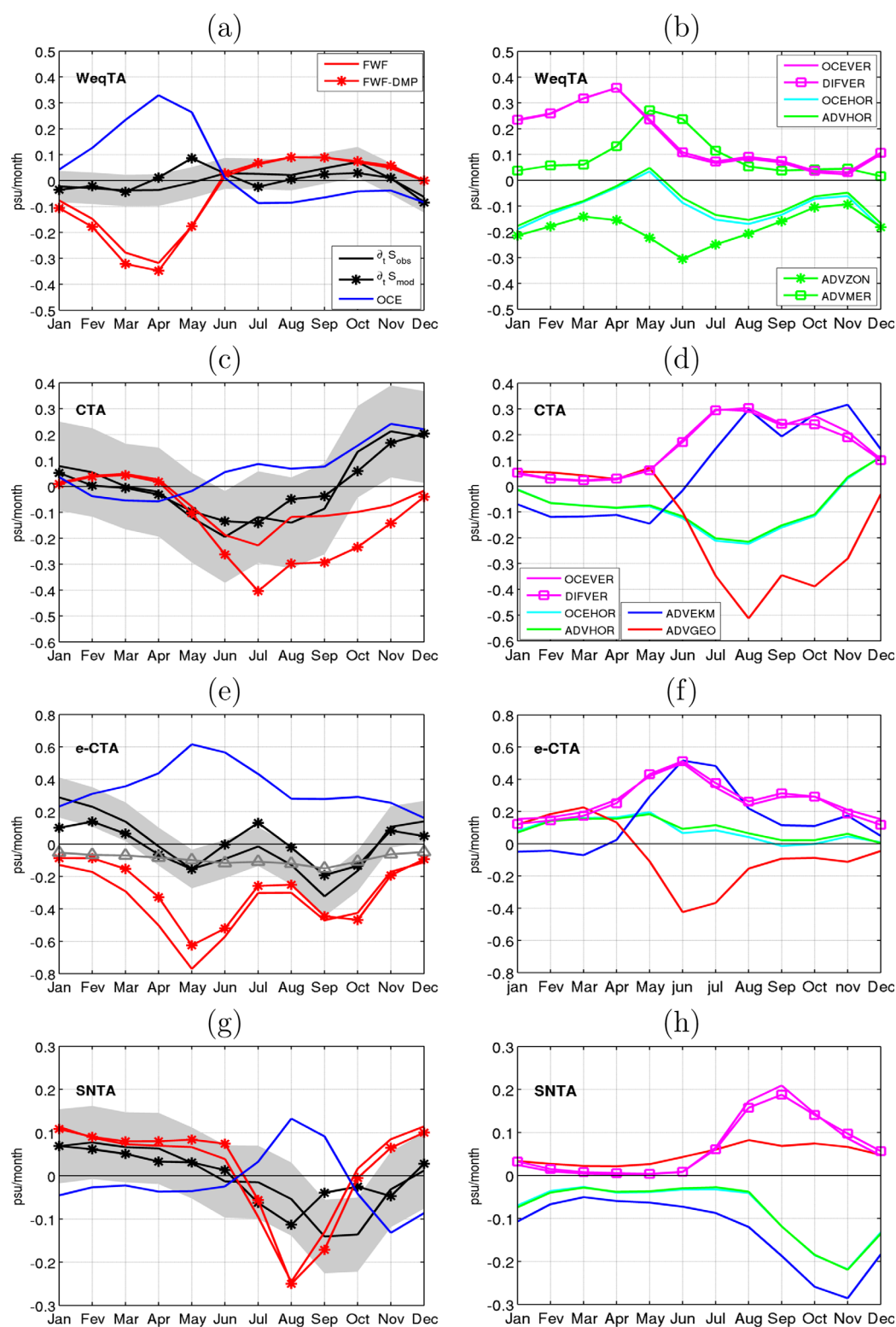
Figure 7. As Figure 4 except for (b) where horizontal advection is separated into zonal and meridional components: WeqTA ( 7^{\circ}S;3^{\circ}N/40:15^{\circ}W ), CTA ( 3:10^{\circ}N/48:20^{\circ}W ), e-CTA ( 3:10^{\circ}N/20:14^{\circ}W ), and SNTA ( 10:17^{\circ}N/48:20^{\circ}W ).
