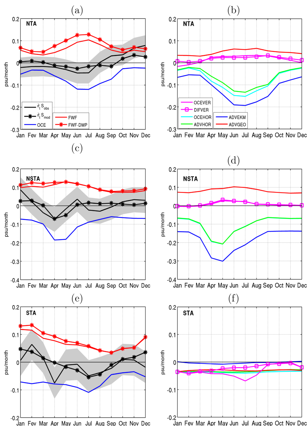
Figure 4. Seasonal evolution of the (a, c, and e) mixed layer salinity budget and (b, d, and f) its components due to ocean dynamics in psu/month averaged over: (Figures 4a and 4b) the NTA region (17:25°N/58:20°W), (Figures 4c and 4d) the NSTA region (13:7°S/35°W:8°E), and (Figures 4e and 4f) the STA region (25:13°S/35 degree W:8°E). In Figure 4d, the cyan curve is overlaid by green line curve. The shaded areas show the estimation of error on data (see text for details). Definitions of the colored lines are given in the legend of the top plot, see text for details.
