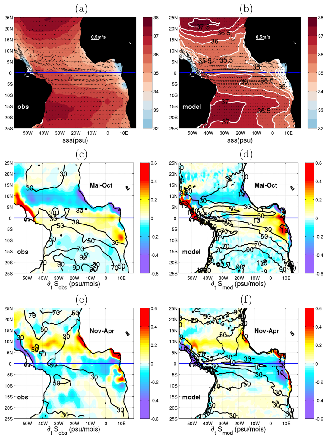
Figure 1. Annual mean SSS (colors, in practical salinity unit (psu)) and surface currents (arrows, in m/s) from (a) observations and (b) the model. White contours in Figure 1b represent the model salinity averaged over the mixed layer depth. (center) May–October mean MLS tendency (colors in psu/mois) and mixed layer depth (contours in m) from (c) observations and (d) the model. (e, f) Same as Figures 1c and 1d for the November–April mean.
